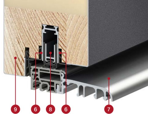
cross-section of the THERMO HOT 78 leaf with and without drop down gasket, aluminium threshold
