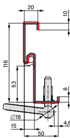
CORNER STEEL FRAME
