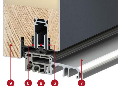
cross-section of the THERMO 64 leaf with and without drop down gasket, aluminium threshold
