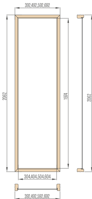
Side lights for fixed door frame
