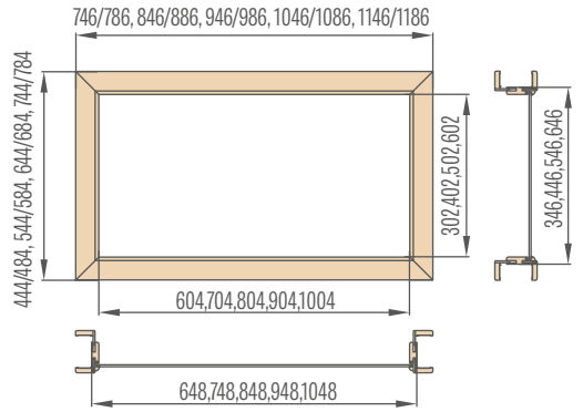
Top lights for adjustable door frame in rebated double doors architrave 6 cm/architrave 8 cm
