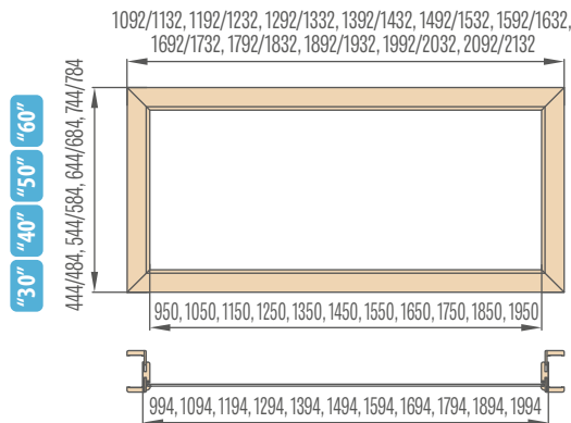
Top lights for adjustable door frame in rebated double doors architrave 6 cm/architrave 8 cm
