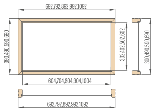
Top lights for fixed door frame in single doors
