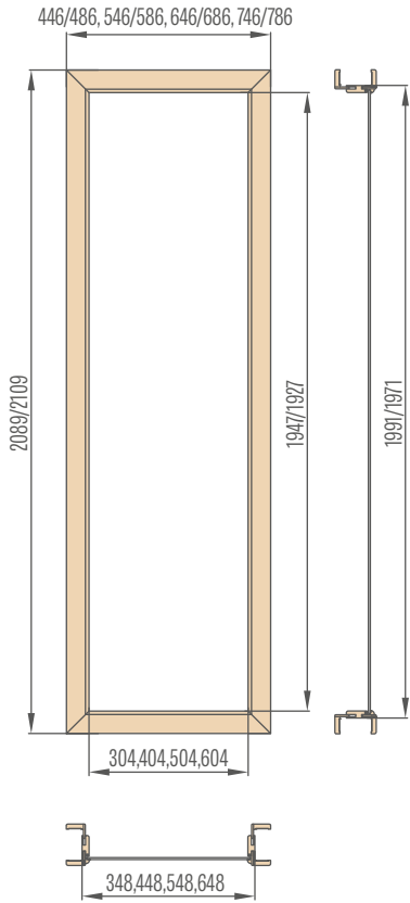
Side lights for rebated adjustable door frame Architrave 6 cm/architrave 8 cm
