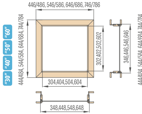
Top lights for adjustable door frame in rebated double doors architrave 6 cm/architrave 8 cm
