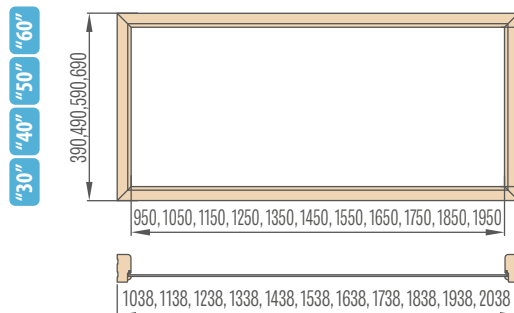
Top lights for fixed door frame in double doors
