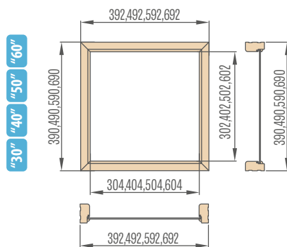
Top lights for fixed door frame in double doors
