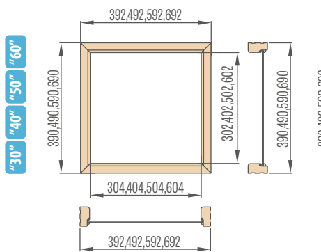
Top lights for fixed door frame in double doors
